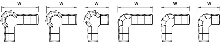
3-Seater (M) W:86 1/4" H:40 1/4" - 44" D:35" 3-Seater (L) W:96 3/4" H:40 1/4" - 44" D:35" Seat height: 18" 3-Seater (M) W:86 1/4" H:33 3/4" D:35" 3-Seater (L) W:96 3/4" H:33 3/4" D:35" Seat height: 18"
