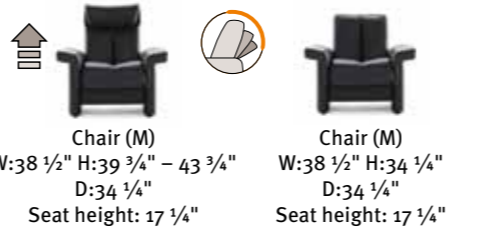
Chair (M) W:38 1/2" H:39 3/4" - 43 3/4" D:34 1/4" Seat height: 17 1/4" Chair (M) W:38 1/2" H:34 1/4" D:34 1/4" Seat height: 17 1/4"
